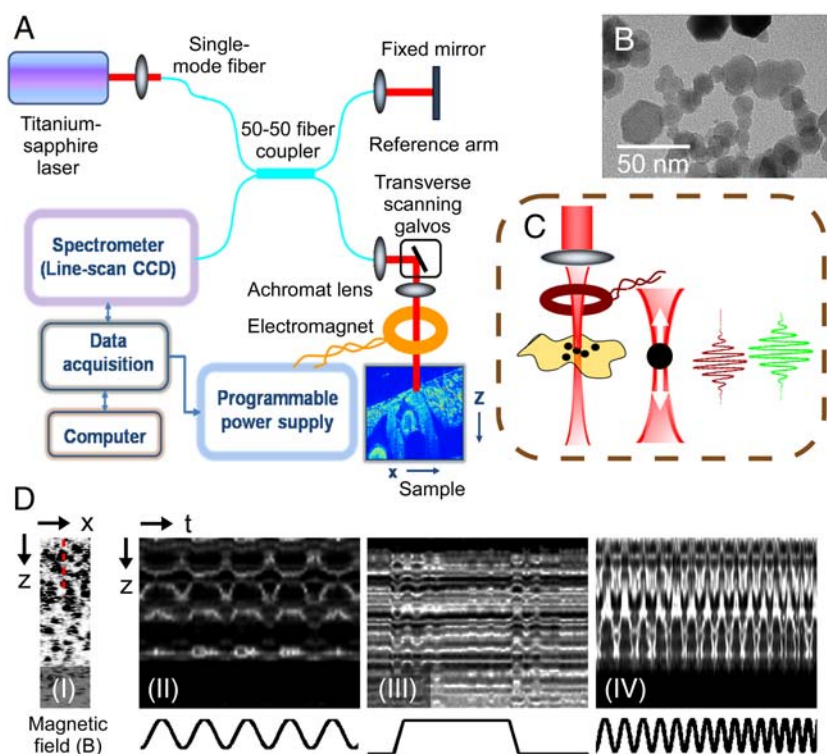
Fig. 1. MM-OCT principle. (A) Schematic of the experimental setup. (B) TEM of the MNPs used in the study. (C) Close-up of the sample arm with focusing lens, electromagnet, and specimen showing axial magnetomotive displacements of MNPs and corresponding change in the OCT interferogram. (D) (I) B-mode image through a MNP-silicone phantom. (II–IV) Representative zoomed-in images of M-mode scans along the dashed red line marked in (I) showing magnetomotion in the sample on application of a (II) sinusoidal, (III) pulse, and (IV) sweep of frequencies of the magnetic field.
