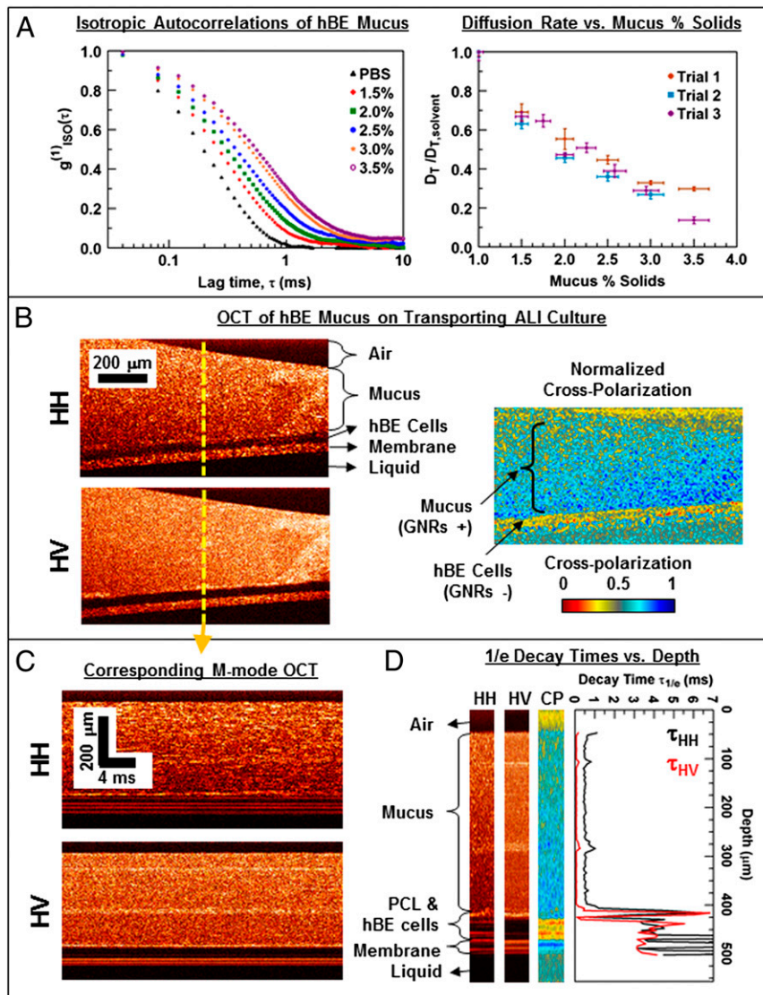
Fig. 4. GNR diffusion in stationary mucus (A) and in actively transporting hBE mucus in an ALI culture (B–D). (A) GNR diffusion in varying mucus percentage solids (where the solvent is 1× PBS at 1% solids). (Left) Representative isotropic autocorrelations. (Right) Corresponding relative diffusion rates D_T/D_{T,\text{solvent}} ( n \geq 6 ; average and SD; three independent trials plotted). GNR diffusion is significantly hindered as the mucus solids concentration increases. (B) Representative HH , HV , and CP OCT images of mucus [2.5% (wt/wt) solids] with GNRs on a transporting ALI culture. A layer devoid of GNRs corresponding to hBE cells exhibits low cross-polarization in comparison with GNRs within the mucus layer. (C) A portion of the M-mode OCT data corresponding to the central A-lines of B illustrates more rapid fluctuations in HV compared with HH . (D) Depth-resolved \tau_{HH} and \tau_{HV} corresponding to C discriminates diffusing GNRs within the mucus from slower motile activities in the PCL and hBE cells. A portion of the HH , HV , and CP M-mode images are shown for comparison of each layer position with the decay rates.
